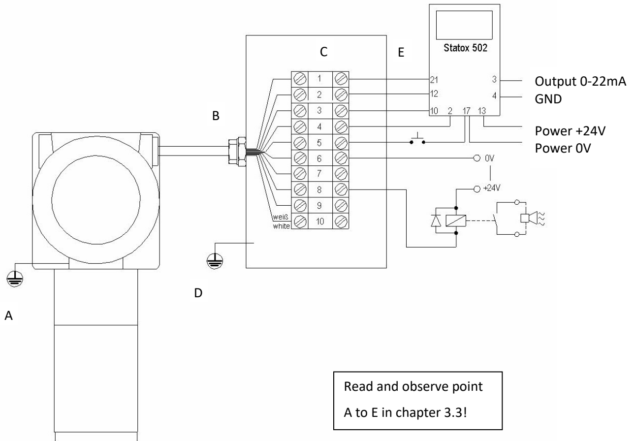
Picture 6: Connect the Stattox 560 to a Stattox 502 Control Module
